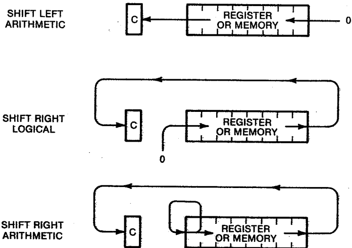
Fig. 12-4. The SHIFT operations.
